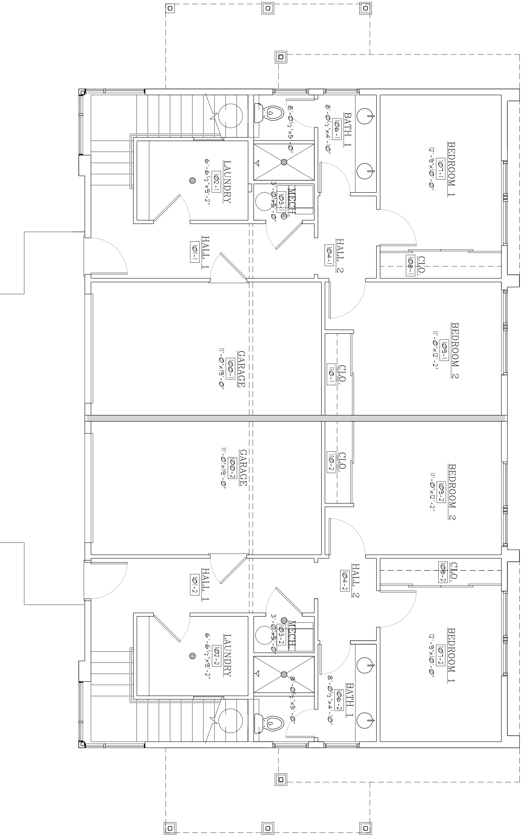
LOT D5 - GROUND FLOOR PLAN
